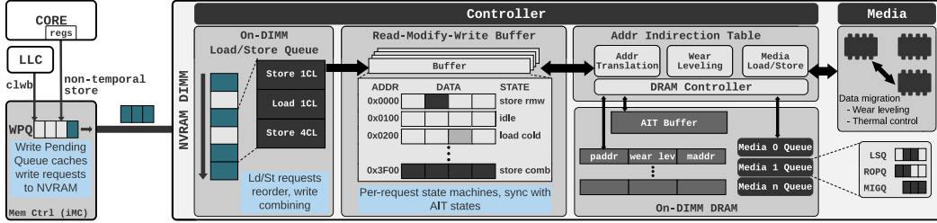
Fig. 8. VANS overview.
