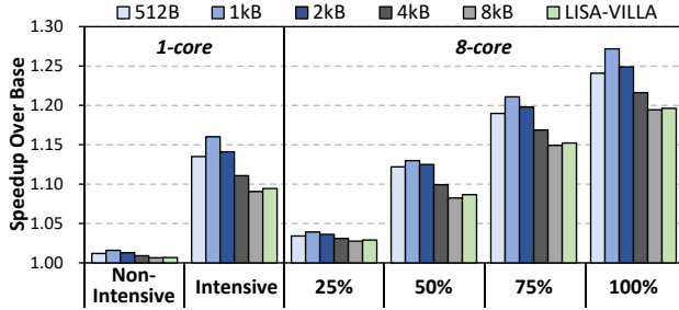
Figure 13. Performance with different row segment sizes.
