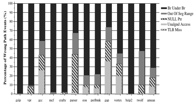
Figure 7. Distribution of wrong-path events.
